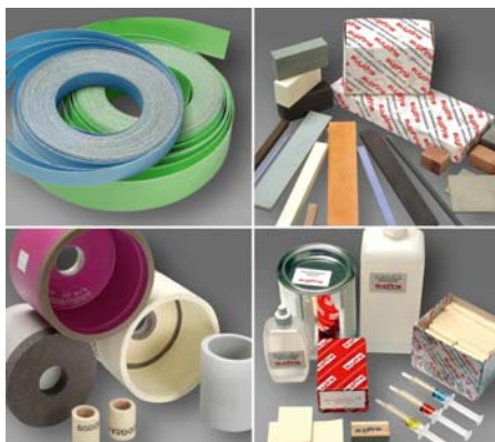
Fig. 6 Supfina superfinishing tools Overview
