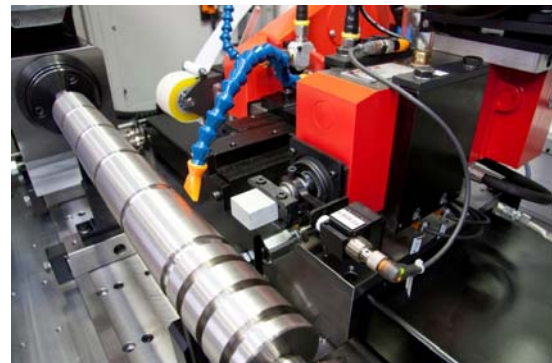
Fig. 2 Supfina Lean Cost Machine® Machine space
